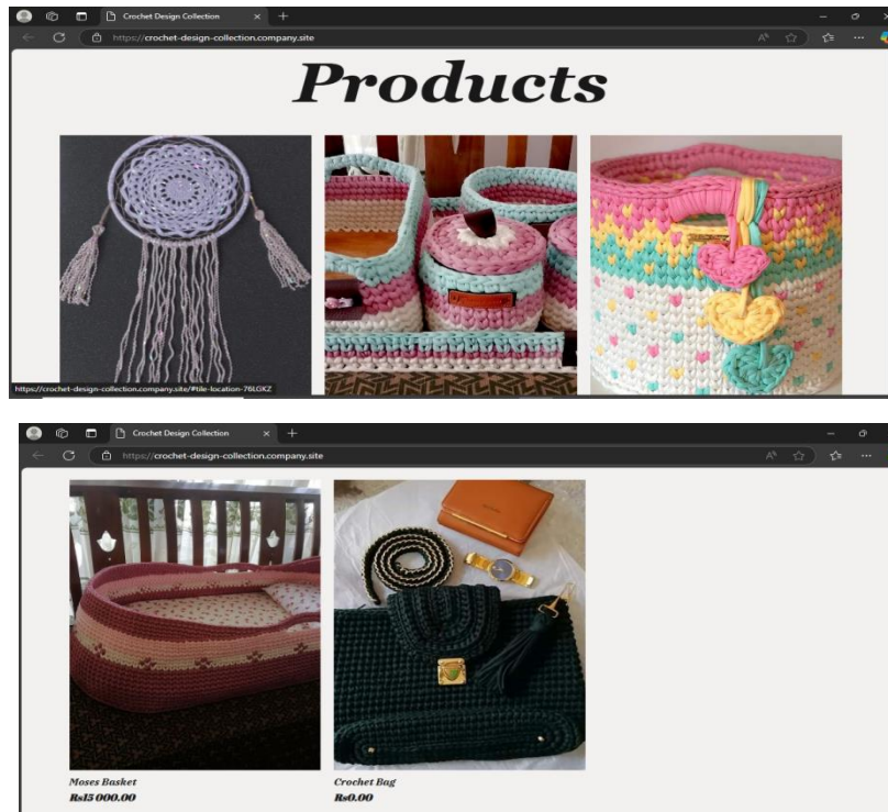
Figure 09- Product
