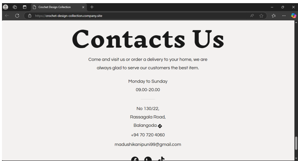
Figure 13- Contact Page
