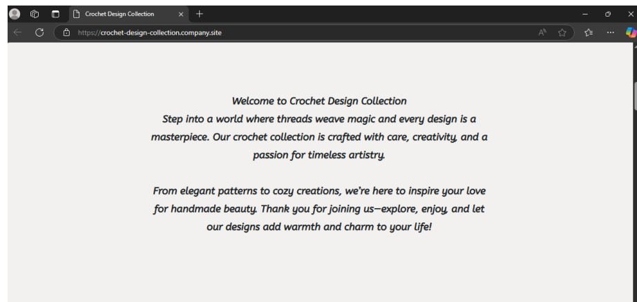
Figure 07- About Page
