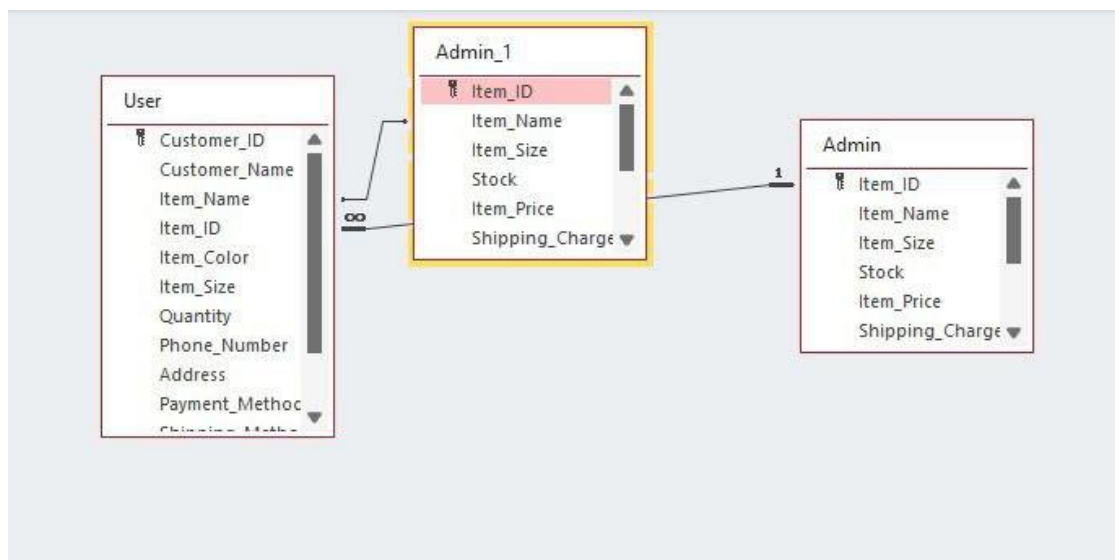
Figure 35- Relationship
