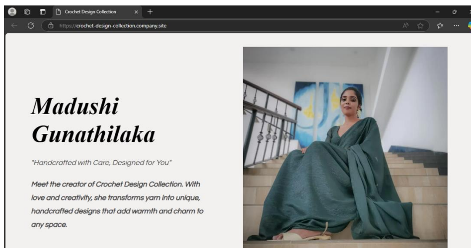
Figure 11- Business Owner
