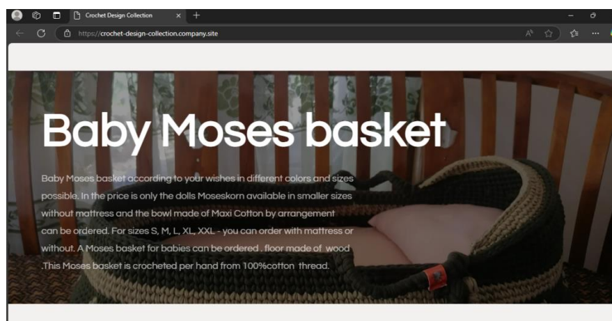
Figure 10- Best Product
