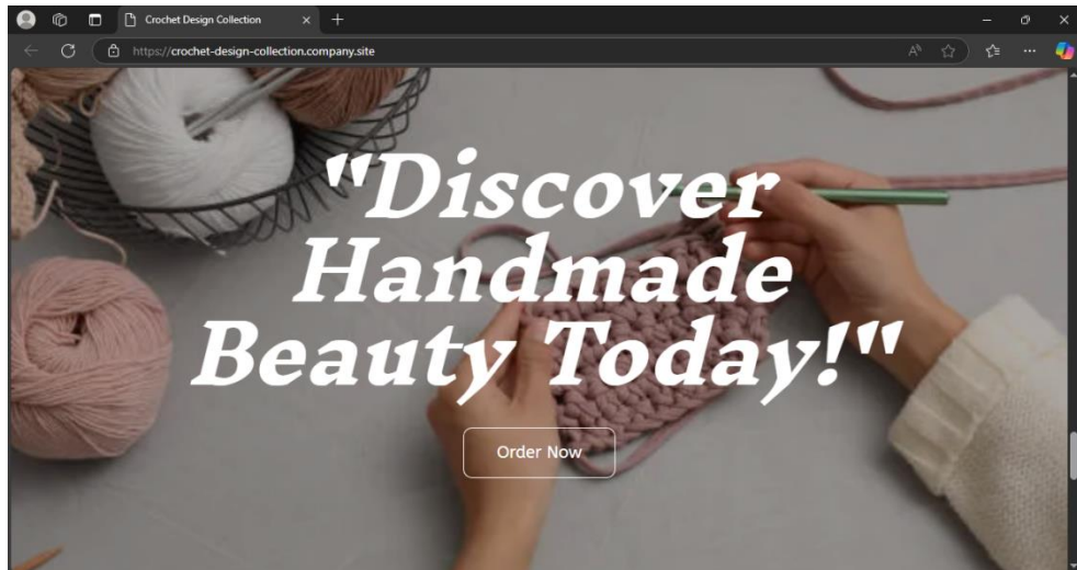
Figure 12- Order Page
