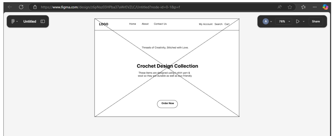
Figure 02- Wire Frame
