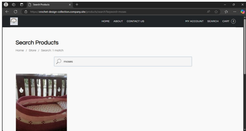
Figure 15- Search Page
