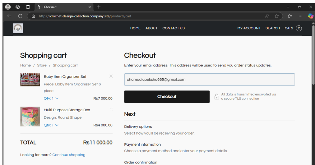
Figure 16- Cart Page
